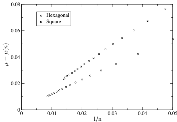
Figure 2. The difference between the connective constant \mu and the lower bound \mu(n) versus 1/n . Data are plotted for the hexagonal and square lattices.
