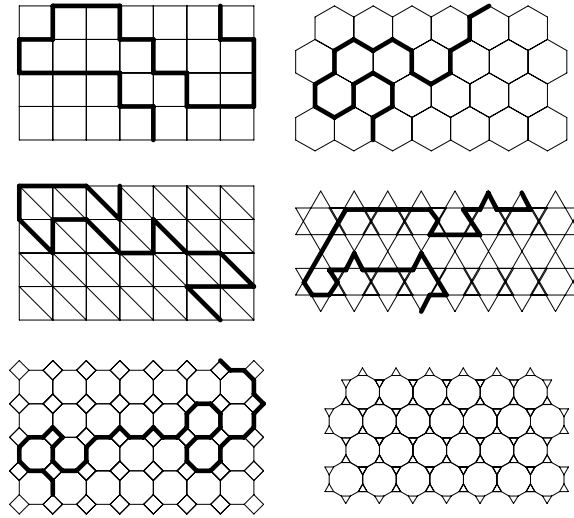
Figure 1. Examples of bridges on the square, hexagonal, triangular, kagomé and (4.8^2) lattices. In addition we also show a section of the (3.12^2) lattice.
